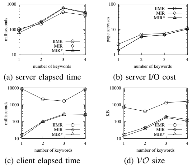
Fig. 11. Performance per Timestamp, Varying the Number of Keywords
