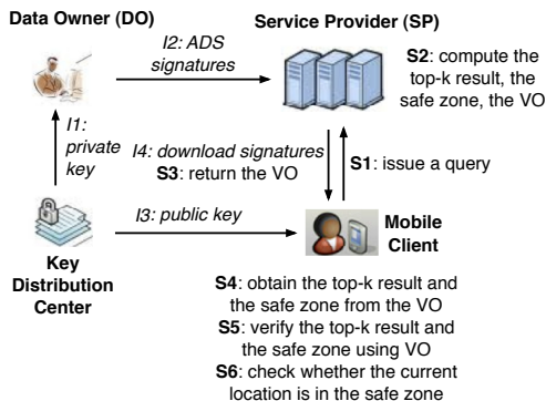
Fig. 2. MkSK Query Authentication
