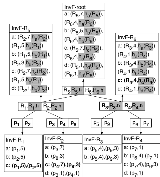
Fig. 3. Example MIR-Tree
