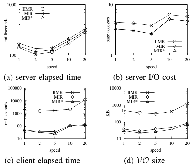
Fig. 12. Performance per Timestamp, Varying the Speed of Moving Queries
